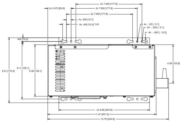
1546 Shelf Mounting
