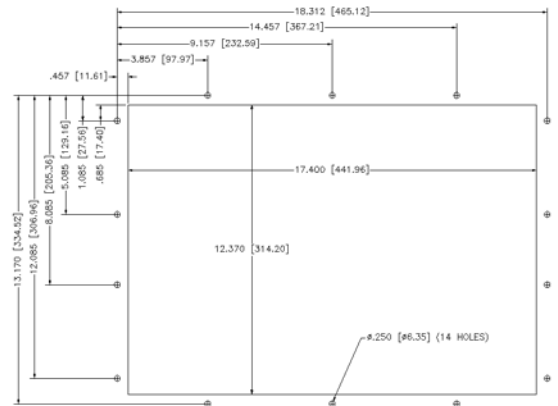
4615KPM(T) Cutout
