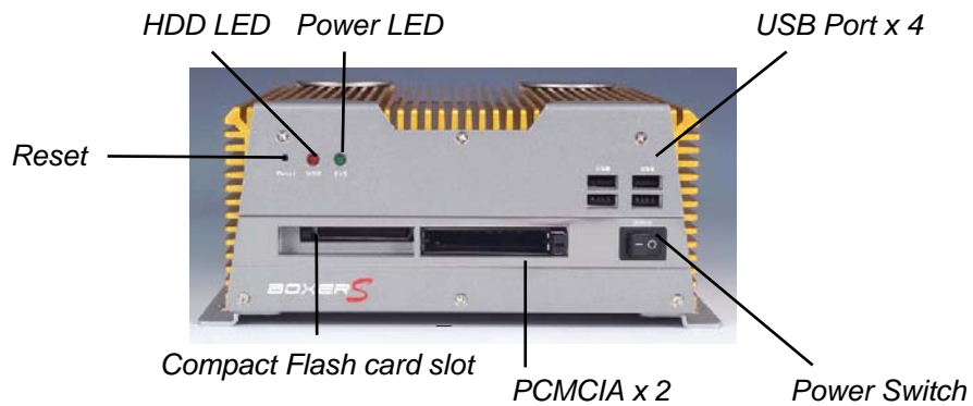
Figure 1-1. Front Side
