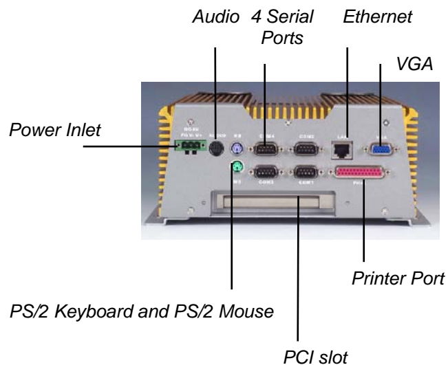
Figure 1-2. Rear Side
